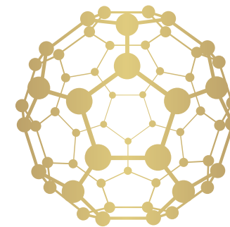
Fullerene C 60
